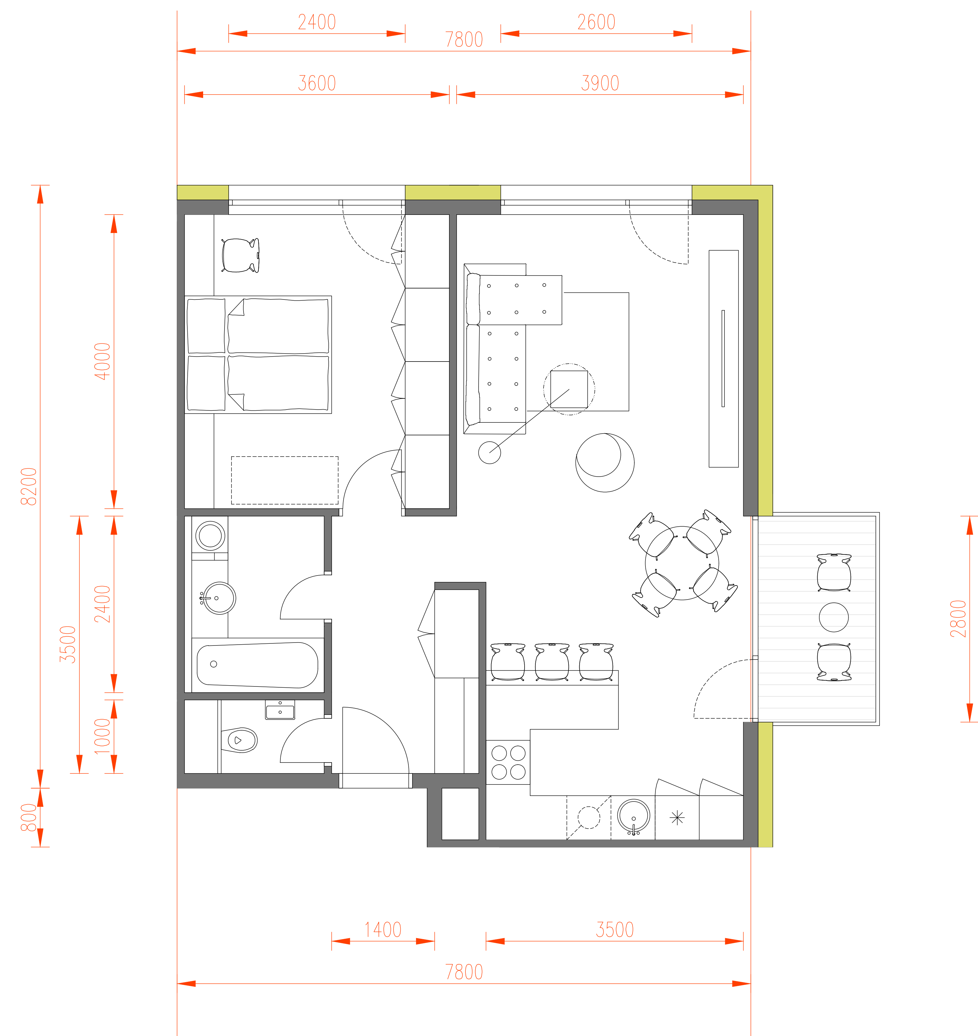
pôdorys 2iR, modul 7,8m 58,54m2 + 4,48m2
