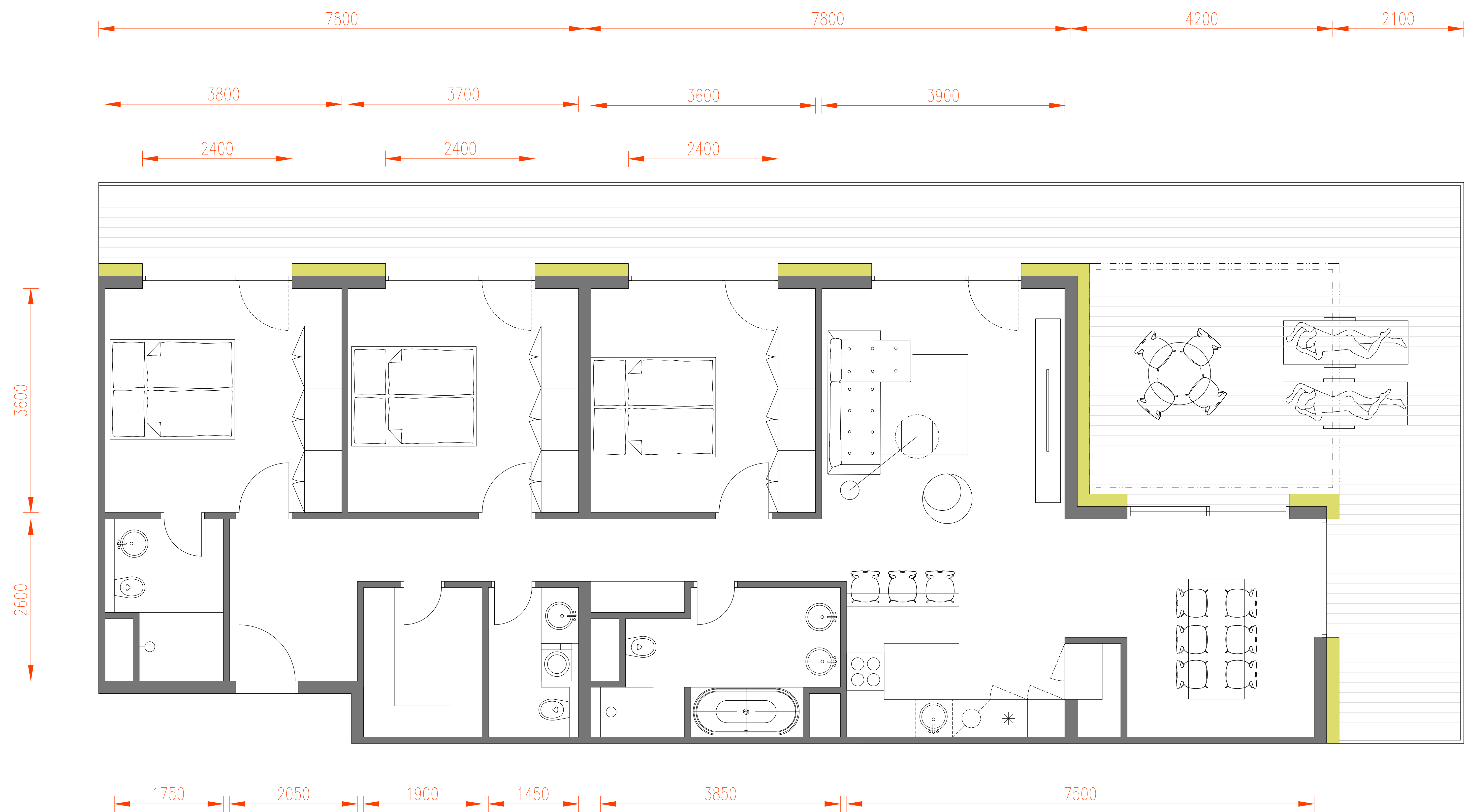
pôdorys 4iR, modul 7,8+7,8+4m 114,54m2 + 59,00m2
