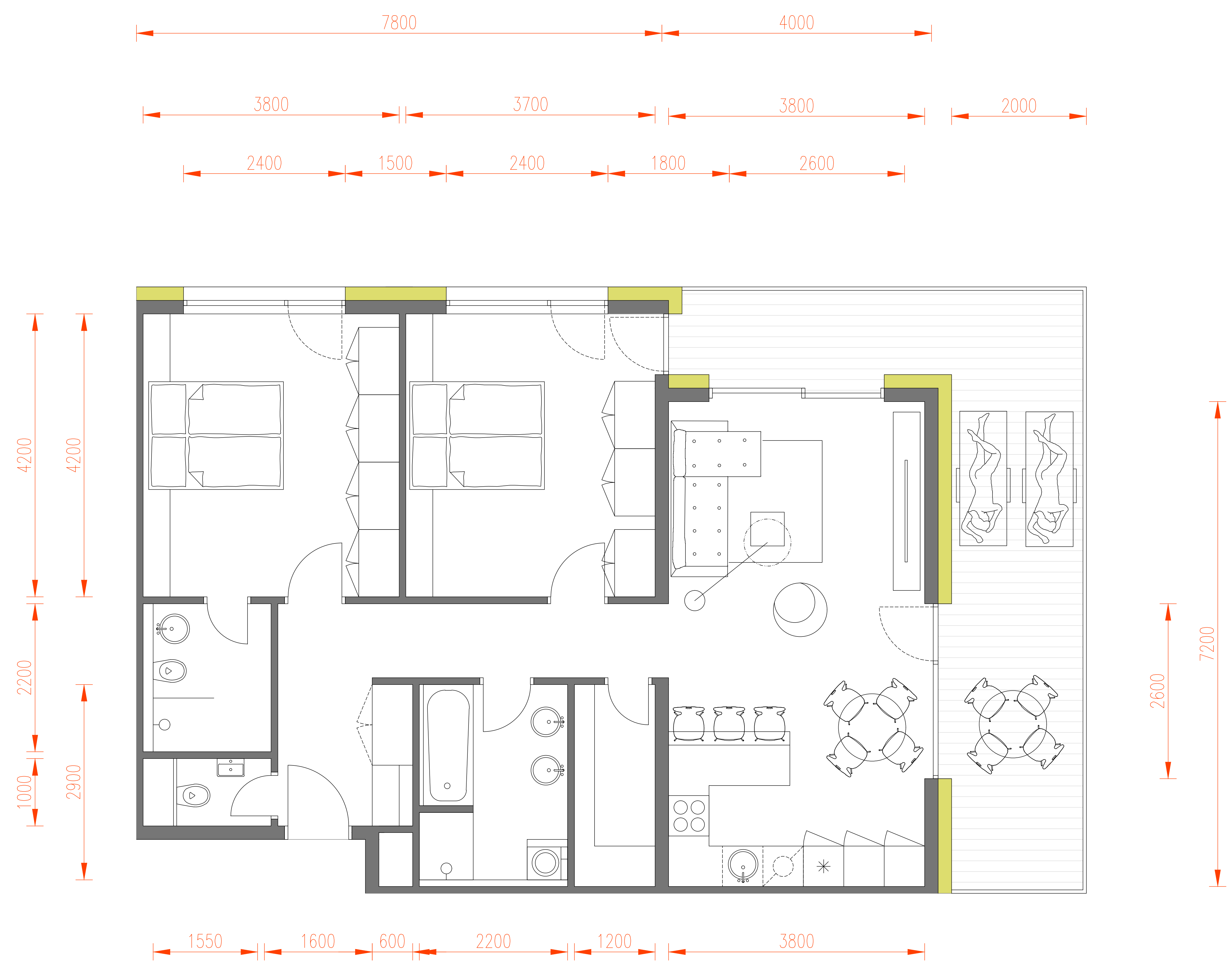
pôdorys 3iR, modul 7,8+4,0m 84,87m2 + 23,20m2
